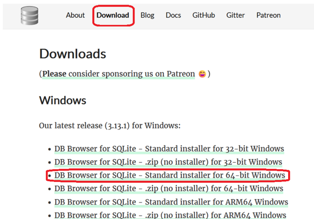
Figure 1: Pobranie instalatora
